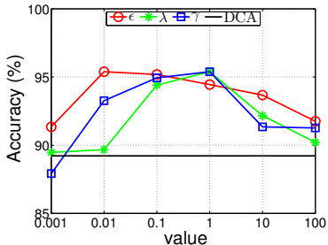
Figure 3: Sensitivity study of SGW on the task C(\text{SURF}) \rightarrow W(\text{DeCAF}_6) w.r.t. parameters \epsilon , \lambda and \gamma .
